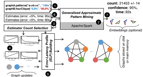
Figure 3: ASAP architecture
