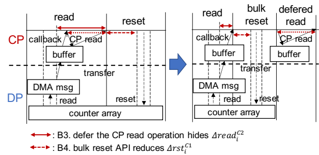
Figure 6: B3: Defer control plane read operation and B4: Use bulk reset API.
